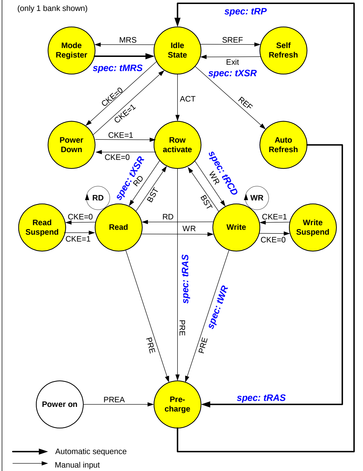
Figure 14: SDRAM configured to full page burst (optional)
