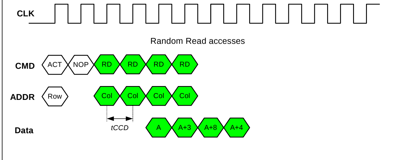
Figure 9: Random Reads, CL=2
