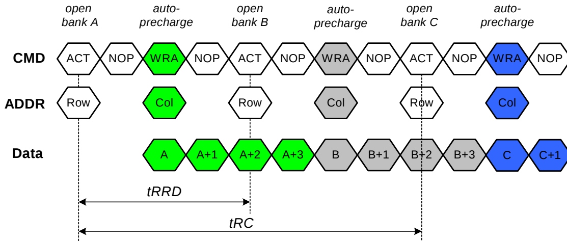
Figure 12: Off page write access for multiple bank activation (BL=4)
